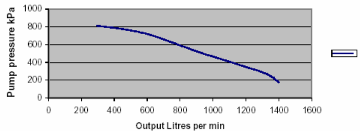
Pump Outputs
